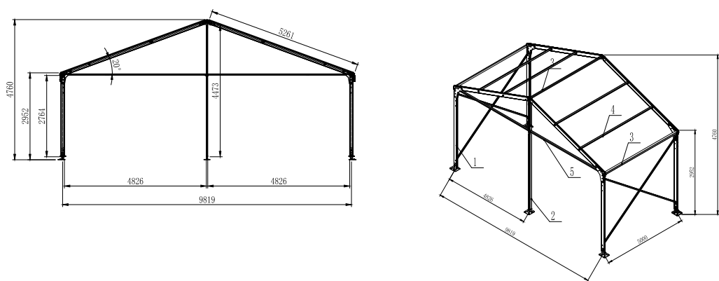
10m Span (5m Bay)
