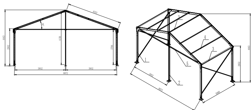
8m Span (5m Bay)
