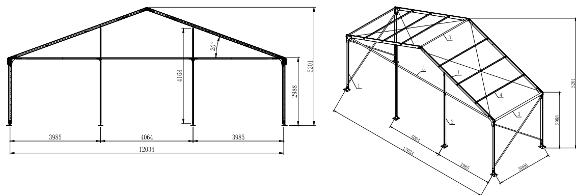
12m Span (5m Bay)
