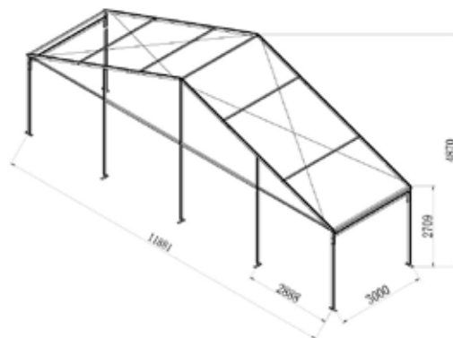
12m GABLE SPAN
