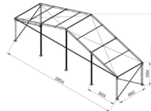
20m GABLE SPAN
