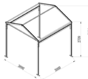
4m GABLE SPAN
