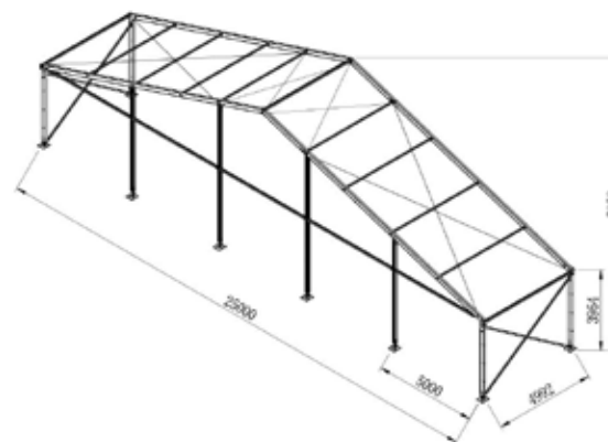
25m GABLE SPAN
