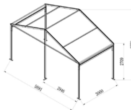
6m GABLE SPAN
