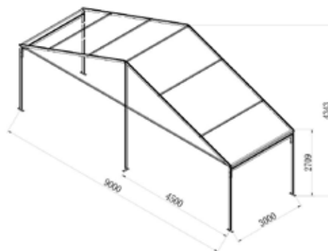
12m GABLE SPAN
