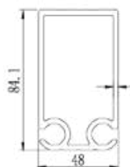
1. Main Profile
