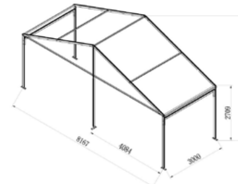
8m GABLE SPAN
