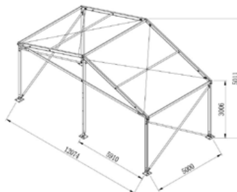
12m GABLE SPAN
