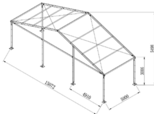
15m GABLE SPAN
