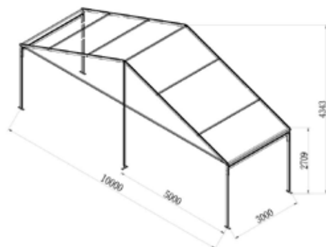
10m GABLE SPAN
