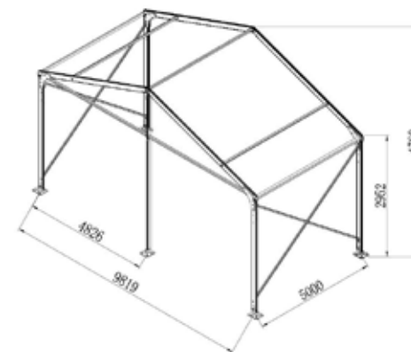
10m GABLE SPAN
