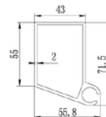
3. Eave Purlin
