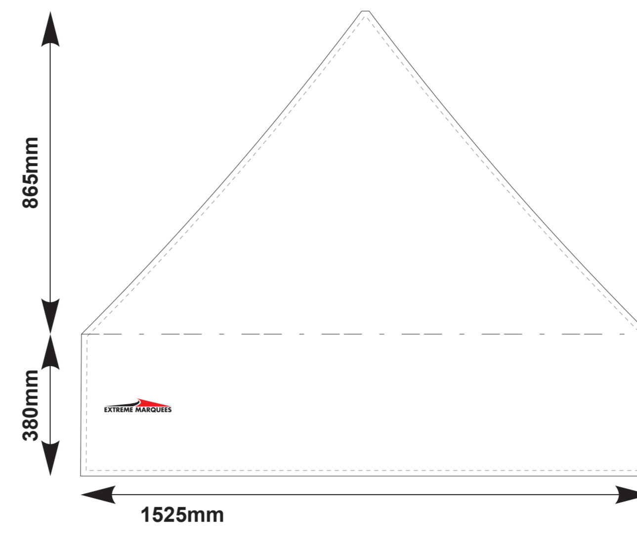
RIGHT VALANCE PANEL
