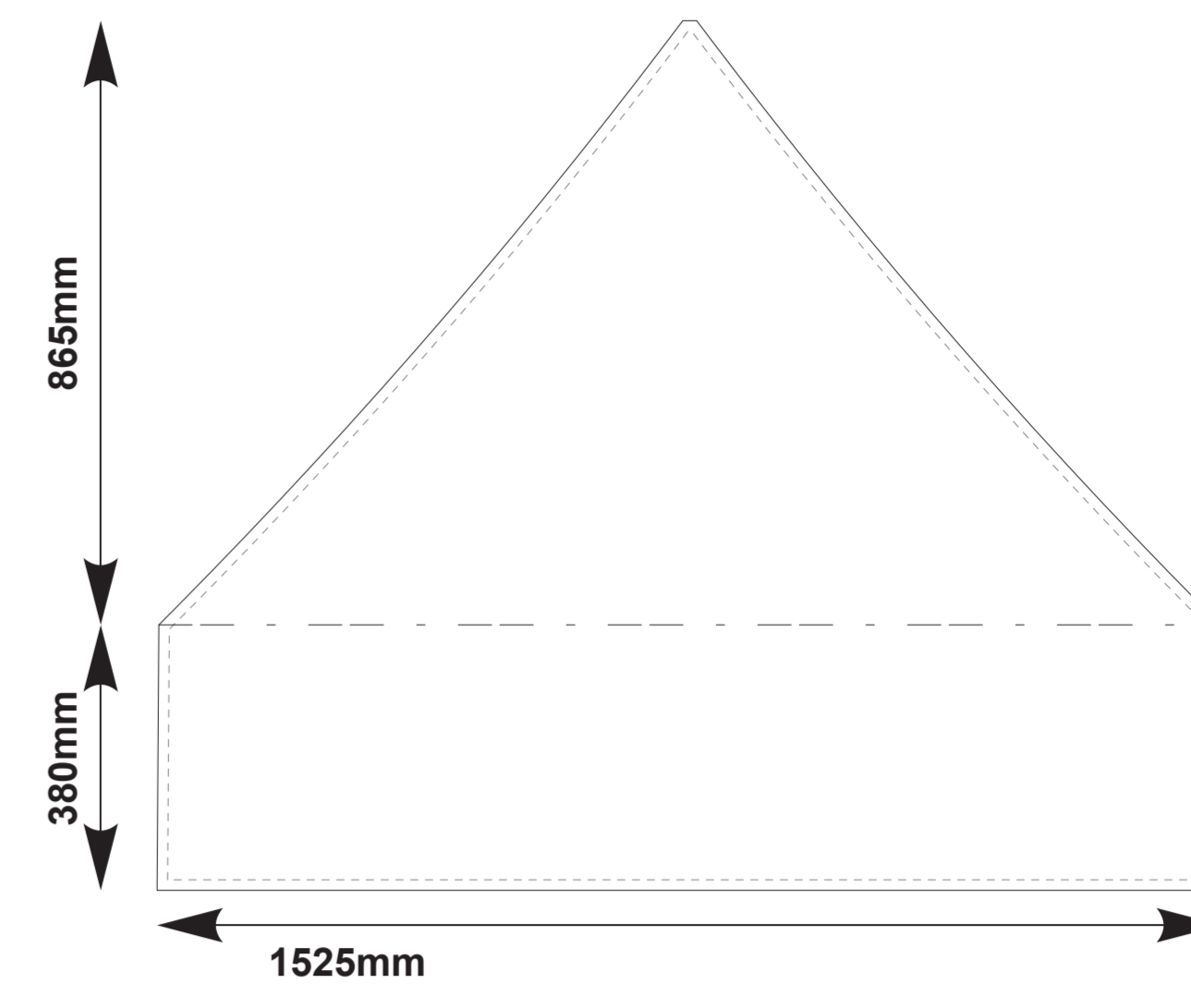
BACK VALANCE PANEL
