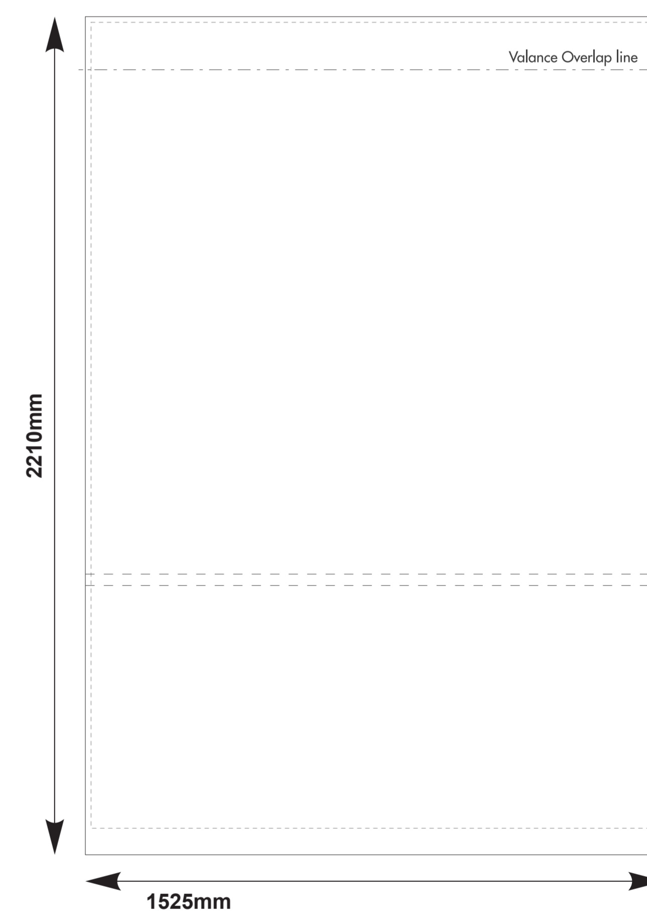
BACK WALL OUTSIDE PANEL
