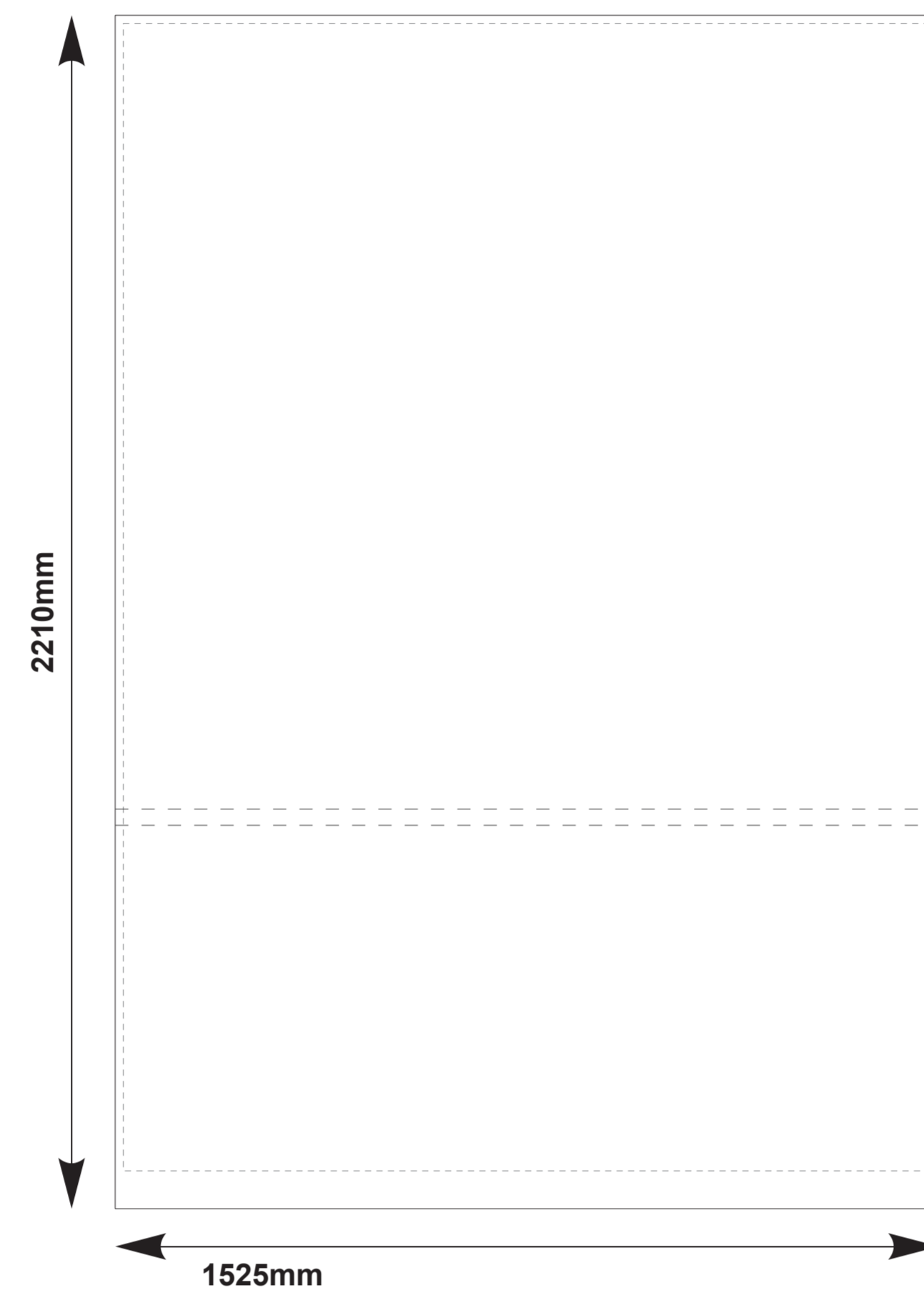
FRONT WALL INSIDE PANEL
